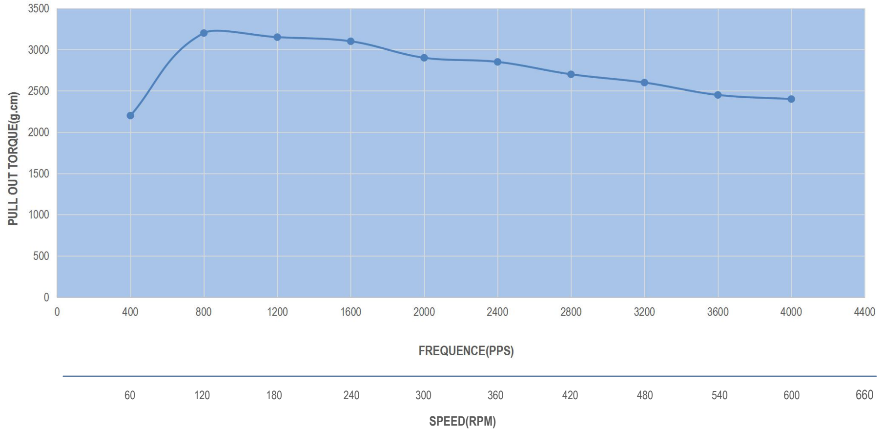
14HS20-1504S PULL OUT TORQUE(1.5A/P 24V HALF STEP /CONSTANT CURRENT)
