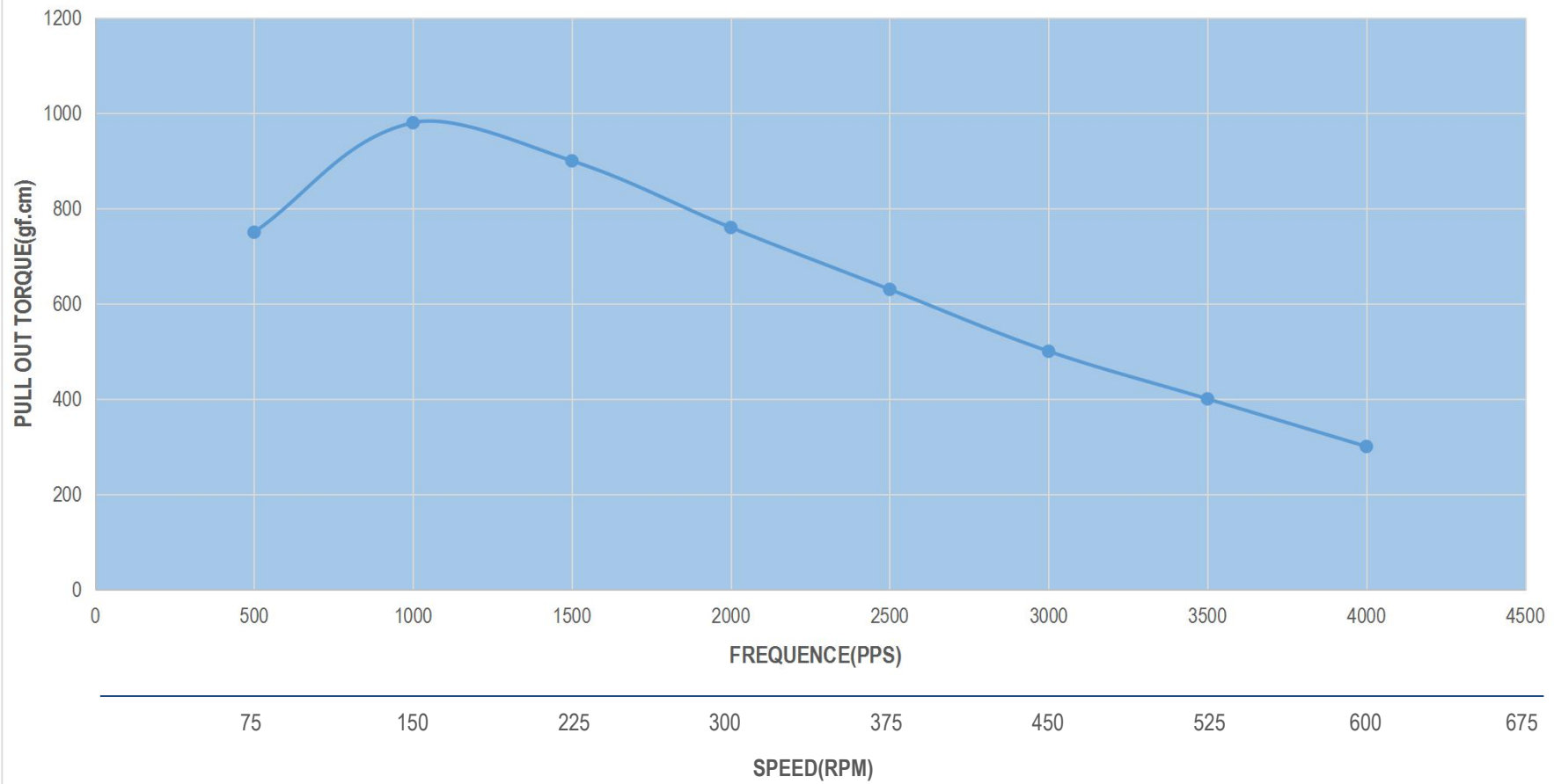
14HS10-0404S PULL OUT TORQUE ( 0.4A/PHASE 24V CONSTANT CURRENT HALF STEP )
