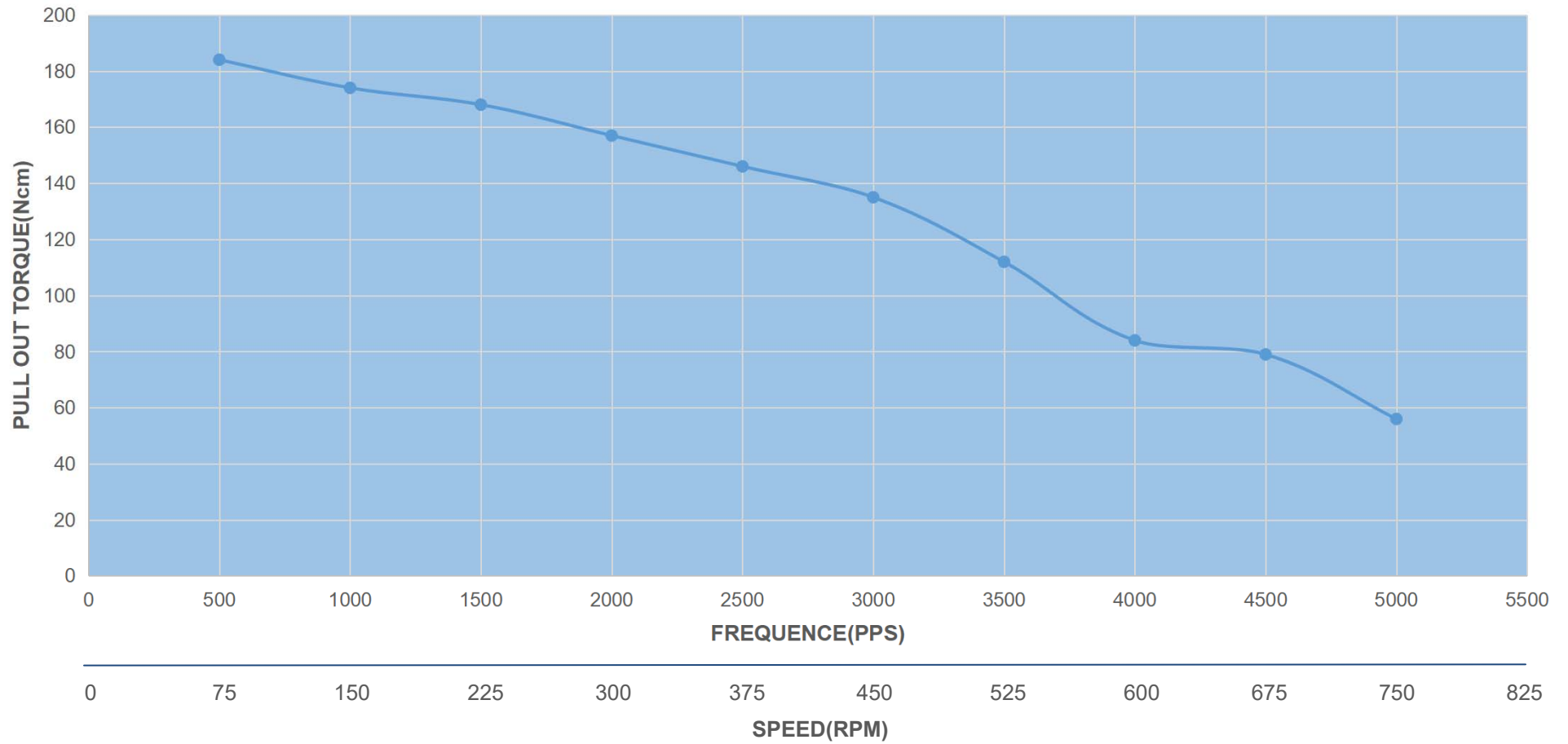
24HS39-3008D PULL OUT TORQUE(4A/P 36V HALF STEP)
