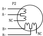
Figure 10: 6-lead motor half coil (higher speed) connections
