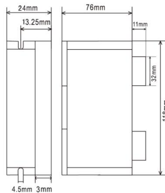
Figure 2: Mechanical specifications
