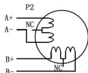
Figure 11: 6-lead motor full coil (higher torque) connections
