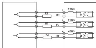
Controller Drive
