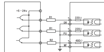
Figure 8: Independent common cathode wiring method
