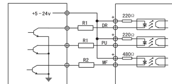
Controller Drive
