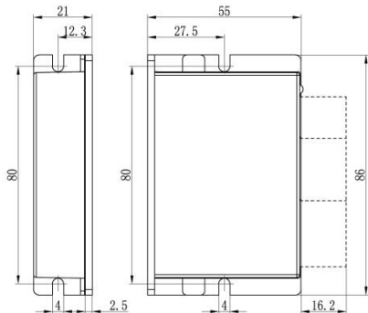
Figure 1: Mechanical specifications
