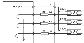
Figure 7: Common anode wiring method
