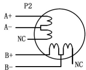
Figure 9: 4-lead Motor Connections
