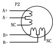
Figure 14: 8-lead motor half coil
