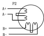
Figure 12: 8-lead motor series connections
