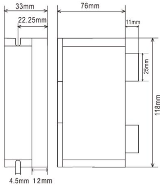
Figure 3: Mechanical specifications
