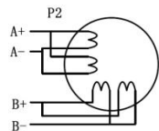
Figure 13: 8-lead motor parallel connections
