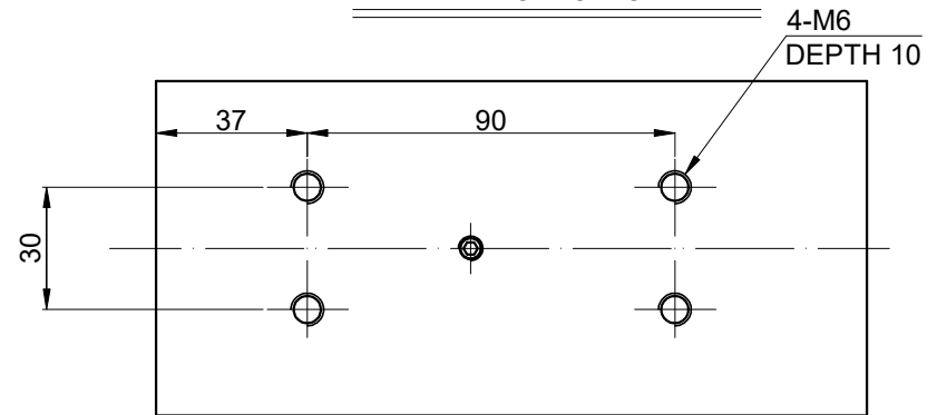
B VIEW BOTTOM OF SHELL
