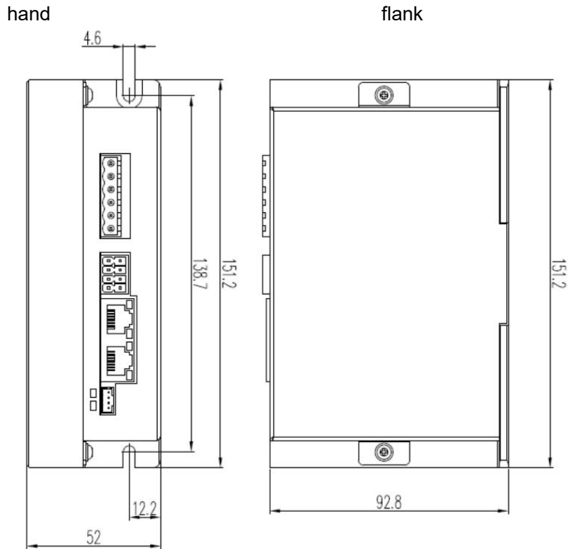
Installation size drawing(unit: mm)
