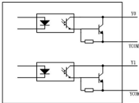
Y0-Y1 output terminal internal circuit
