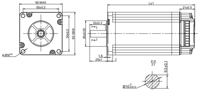
Figure 1: Mechanical specifications
