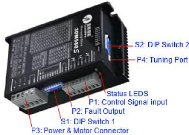
Figure 2 Connectors, DIP switches, and LED locations
