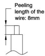
20-6AWG Wires
