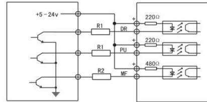
Controller Driver Independent NPN Connection
