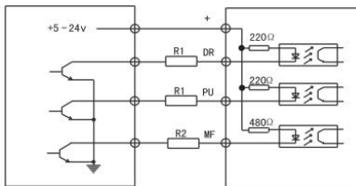
NPN Connection
