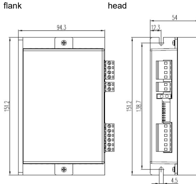
Installation size drawing (unit: mm)
