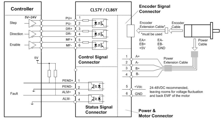
Figure 3: Typical connection
