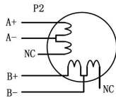
Figure10: 8-lead motor half coil
