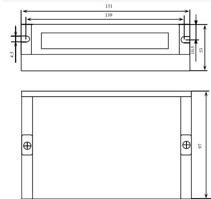
Figure 1 Mechanical specifications
