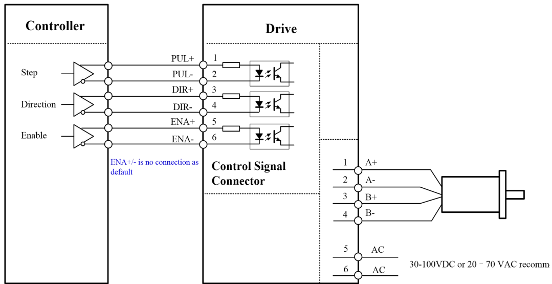
Figure 9: Typical connection
