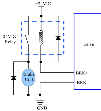
Figure 7: Brake output
