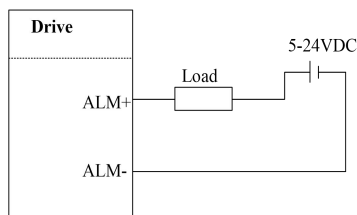
Figure 5: Sinking output
