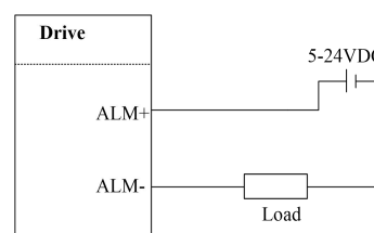
Figure 6: Sourcing output
