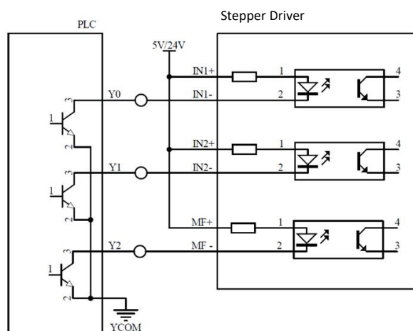
Common positive connection
