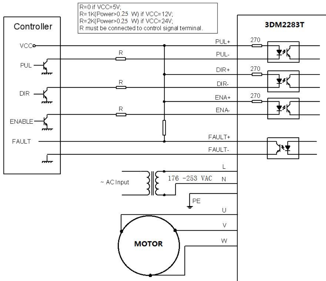
Figure 10: Typical connection
