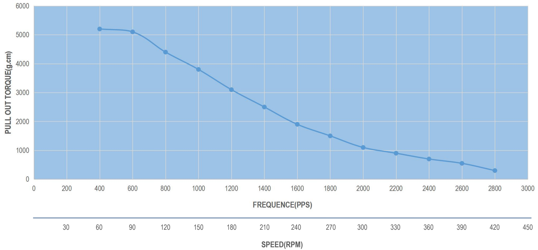
17HS24-0644S PULL OUT TORQUE(0.64A/P 24V HALF STEP)
