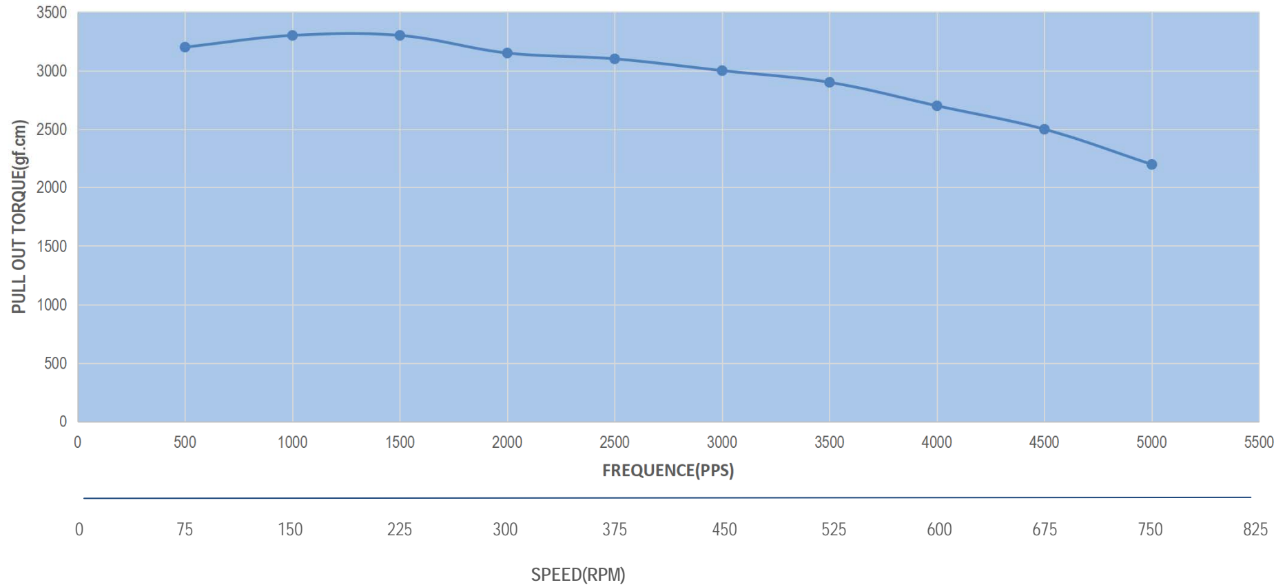
17HS19-1684S-C1 PULL OUT TORQUE ( 1.68A/PHASE 24V CONSTANT CURRENT HALF STEP )
