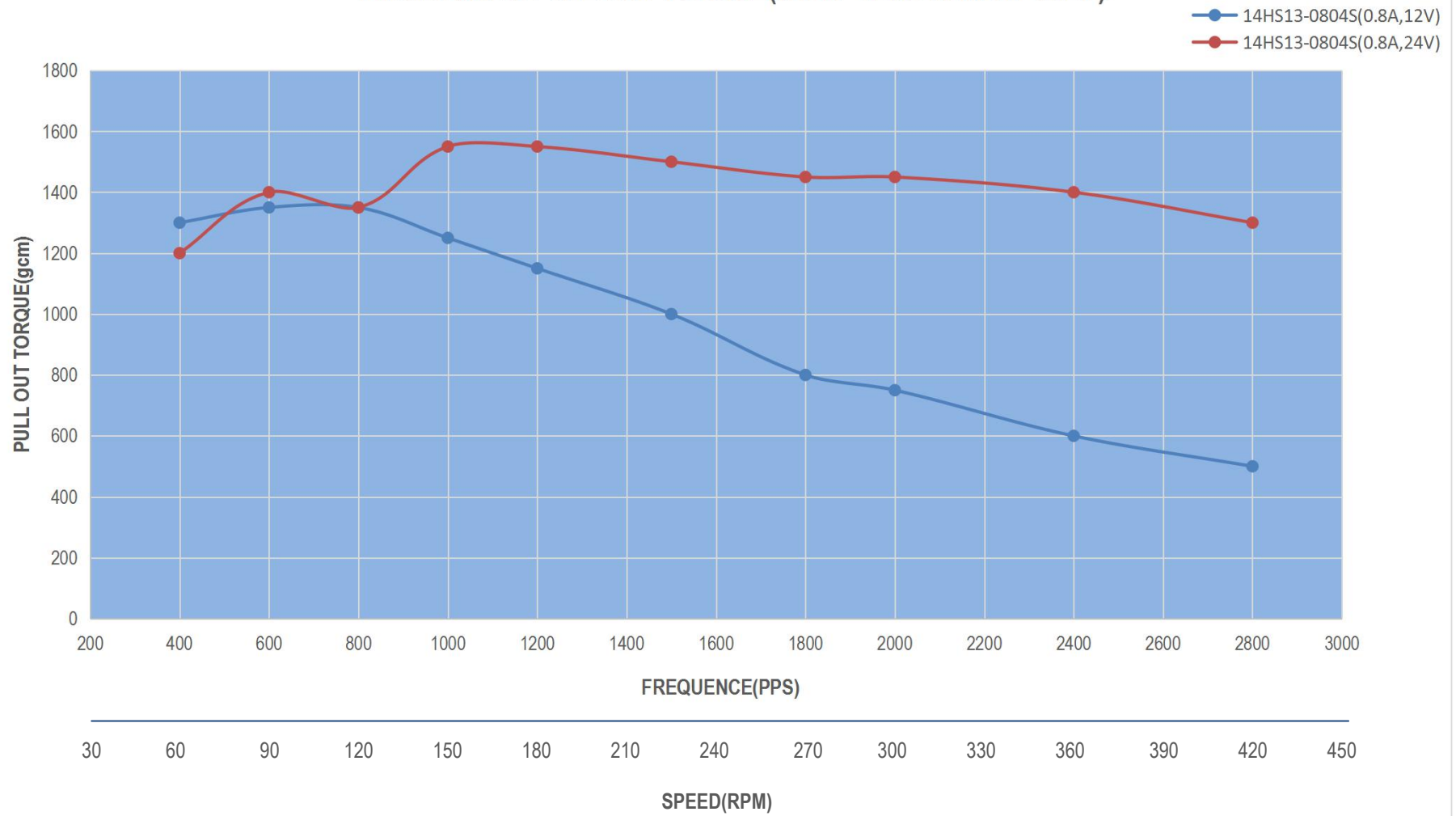
14HS13-0804S PULL OUT TORQUE(0.8A/P 12V/24V HALF STEP)
